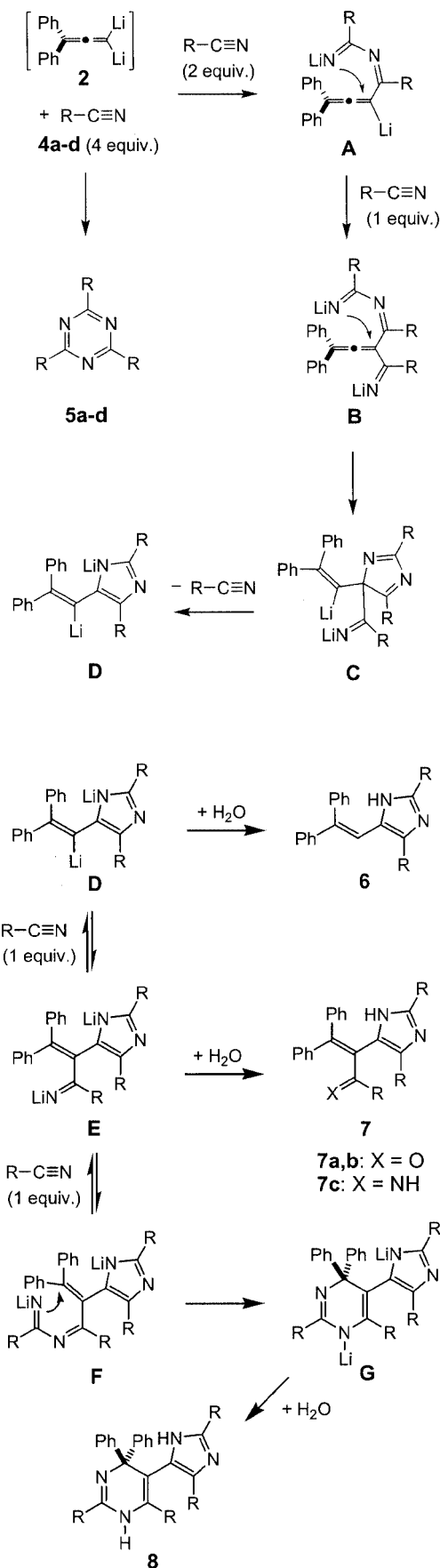
Scheme 3. Reaction between 1,1-dilithio-3,3-diphenylallene and nitriles
