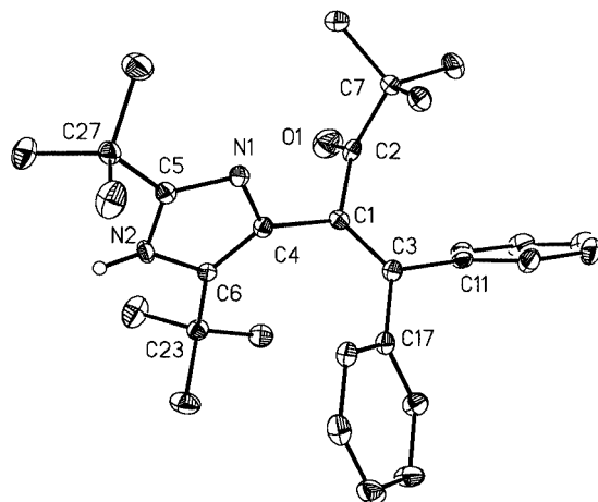
Figure 5. ORTEP plot of 7b ; thermal ellipsoids of 50% probability are shown for the non-hydrogen atoms; selected bond lengths [Å] and angles [°]: O1–C2 1.287(4), N1–C4 1.392(4), N2–C6 1.388(4), C1–C4 1.491(4), N1–C5 1.317(4), N2–C5 1.361(5), C1–C3 1.351(4), C1–C2 1.500(4), C4–C6 1.373(5); C5–N1–C4 105.6(3), C3–C1–C4 125.2(3), C4–C1–C2 113.4(3), O1–C2–C7 118.1(3), C6–C4–C1 132.0(3), N1–C5–N2 110.5(3), C5–N2–C6 109.2(3)
